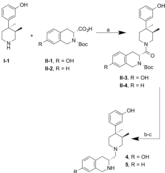
Scheme 2. Synthesis of 4 and 5 a
