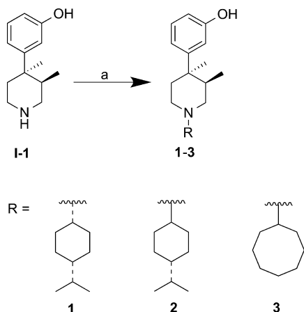
Scheme 1. Synthesis of 1–3 a
